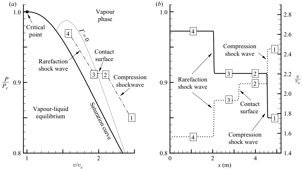
FIGURE 4. One-dimensional numerical solution of the triple-discontinuity shock tube problem under the non-polytropic Martin–Hou model for fluid PP10. States 4 and 1 are the initial state in the high- and low-pressure sections, respectively, see table 2. (a) Solution in the (v, P) -plane together with the saturation curve and the \Gamma = 0 locus. (b) —, reduced pressure P/P_c and . . . , specific volume v/v_c along the shock tube at time t = 29.46 ms. The diaphragm is located at x_{diaph} = 3 m.
