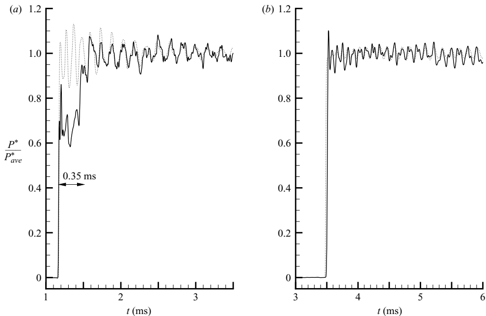
FIGURE 3. Numerical simulation for the partial axisymmetric burst of the diaphragm (· · ·) and experimental results for air in dilute conditions (—). Initial gas state conditions are given in table 1. Results refer to the gauge total pressure P^* measured by probes 1 (a) and 2 (b), located 450 mm ( 5.625 D , where D is the shock tube diameter) and 1650 mm ( 20.625 D ) downwind of the diaphragm position, respectively. P_{ave}^* is the average post-shock gauge total pressure.
